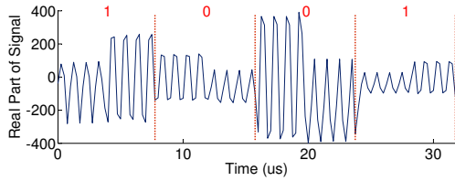
Figure 10—Noisy Reader trace: The eavesdropper’s received signal of the Charlie card communicating with the Noisy Reader still exhibits two clear patterns corresponding to the ‘0’ bits and ‘1’ bits. Despite the random magnitude in each bit and the phase shifting, the eavesdropper can still decode by comparing the first half and the second half of each bit. The ‘0’ bits have the same shape, while the ‘1’ bits have a different one.
