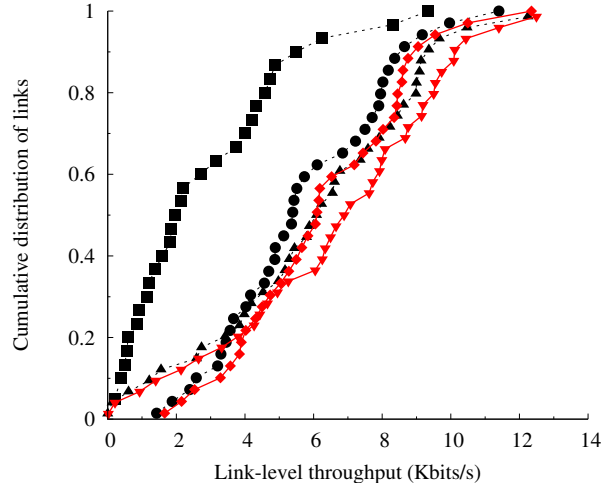
Figure 12: Per-link throughput distribution achieved at the SoftPHY interface. The offered load is 6.9 Kbits/s/node, close to channel saturation.
