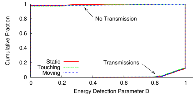
(a) Energy Detection
