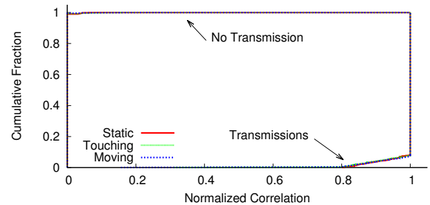
(b) Preamble Correlation
