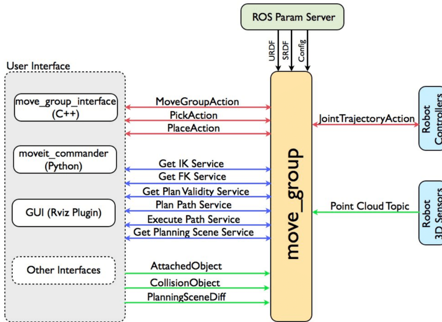
Figure 5: The Schematic Diagram of move group node.
