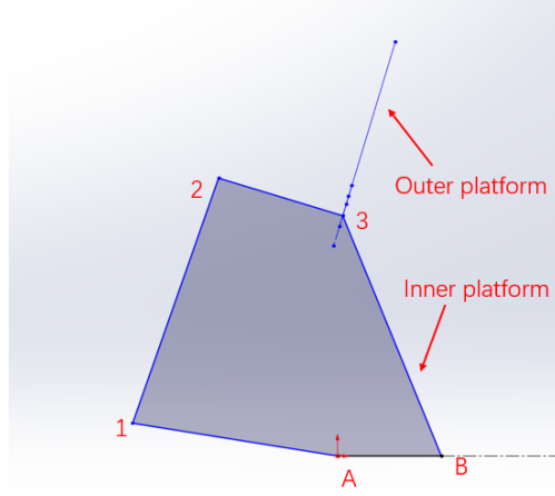
Figure 13: Five-bar linkage
