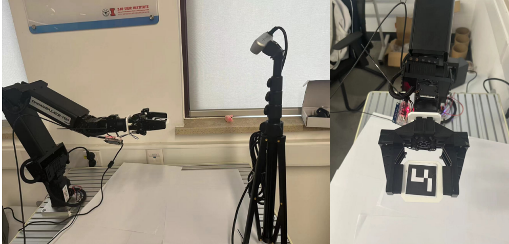
Figure 6: hand-eye calibration.
