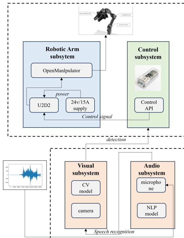
Figure 2: The block diagram of the whole system overview. It contains three subsystems.
