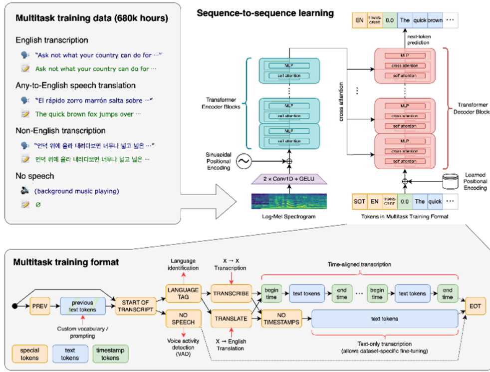
Figure 10: Openai-whisper model.
