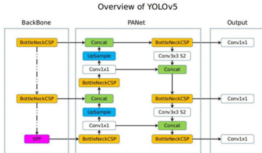
Figure 12: The structure of YoloV5.
