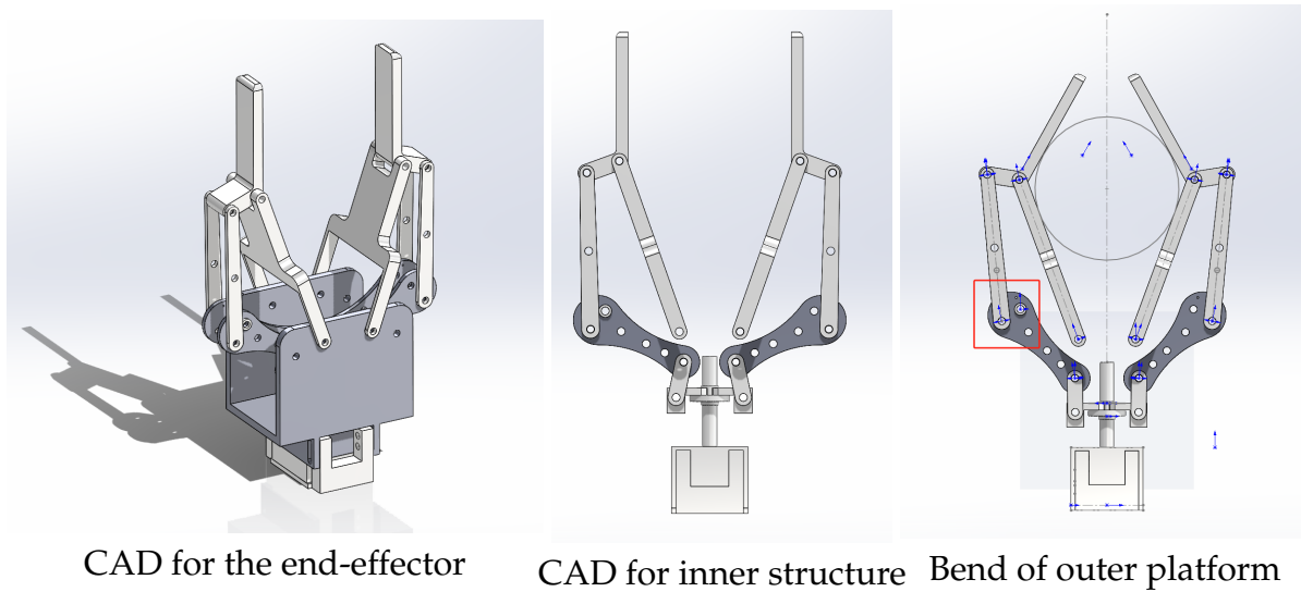
Figure 20: CAD of the end-effector
