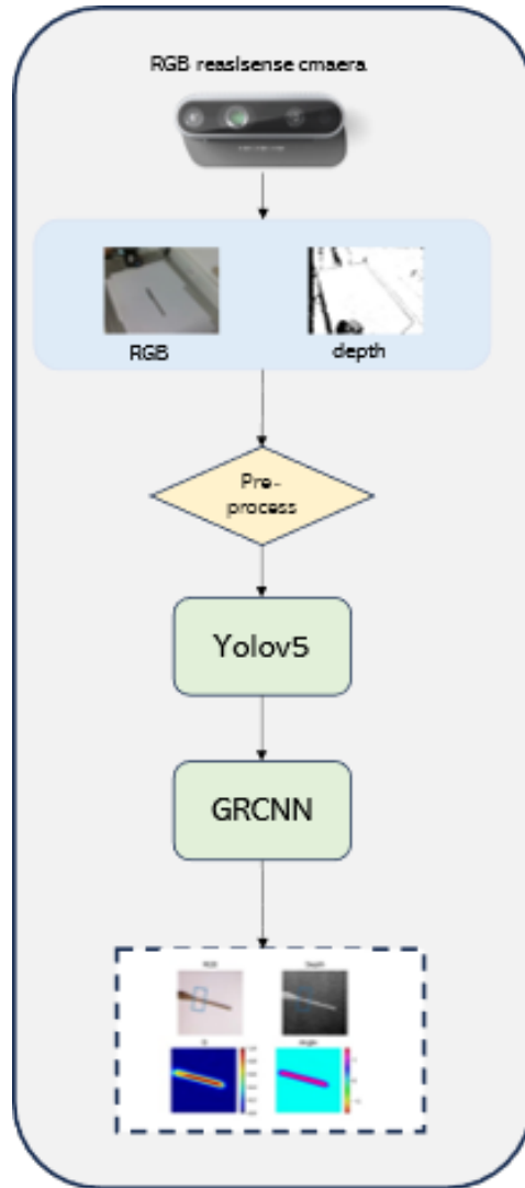
Figure 11: Visual subsystem.
