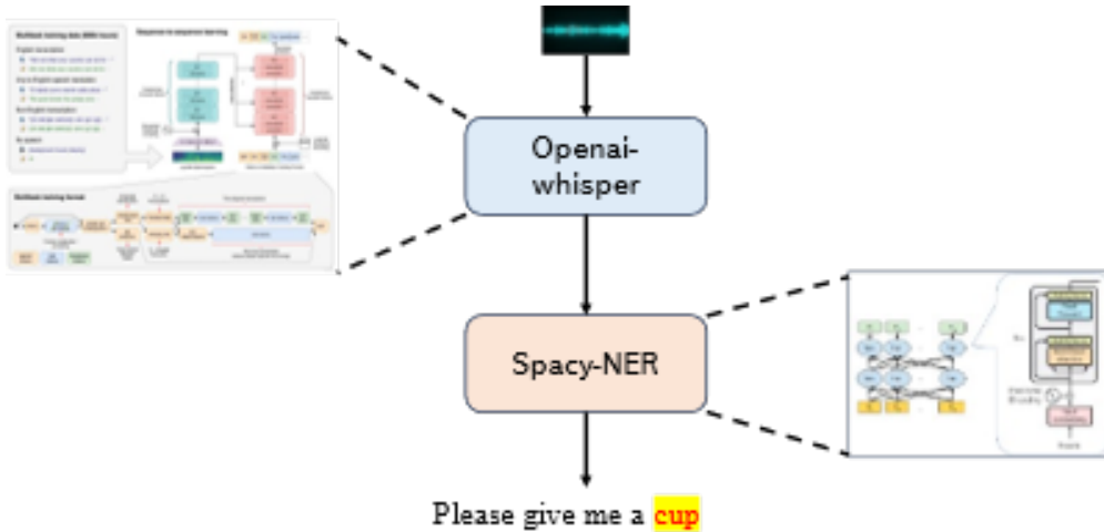
Figure 8: The Control Code.
