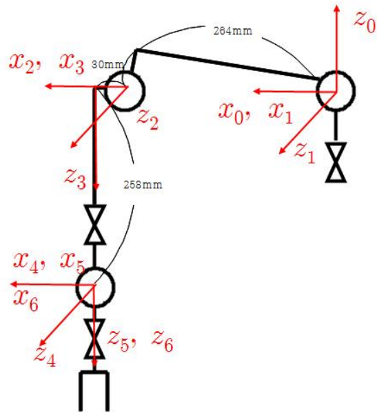
Figure 29: D-H configuration
