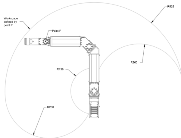
Figure 27: Work space of robotics arm
