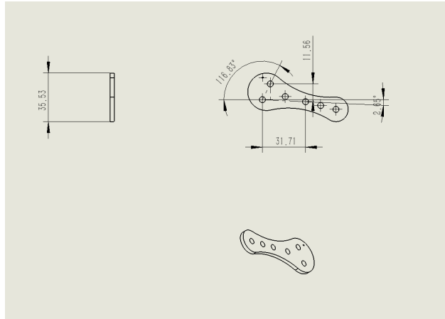
Figure 22: L1 and L2
