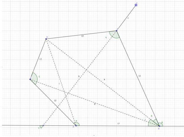
Figure 15: Diagram of five-bar linkage
