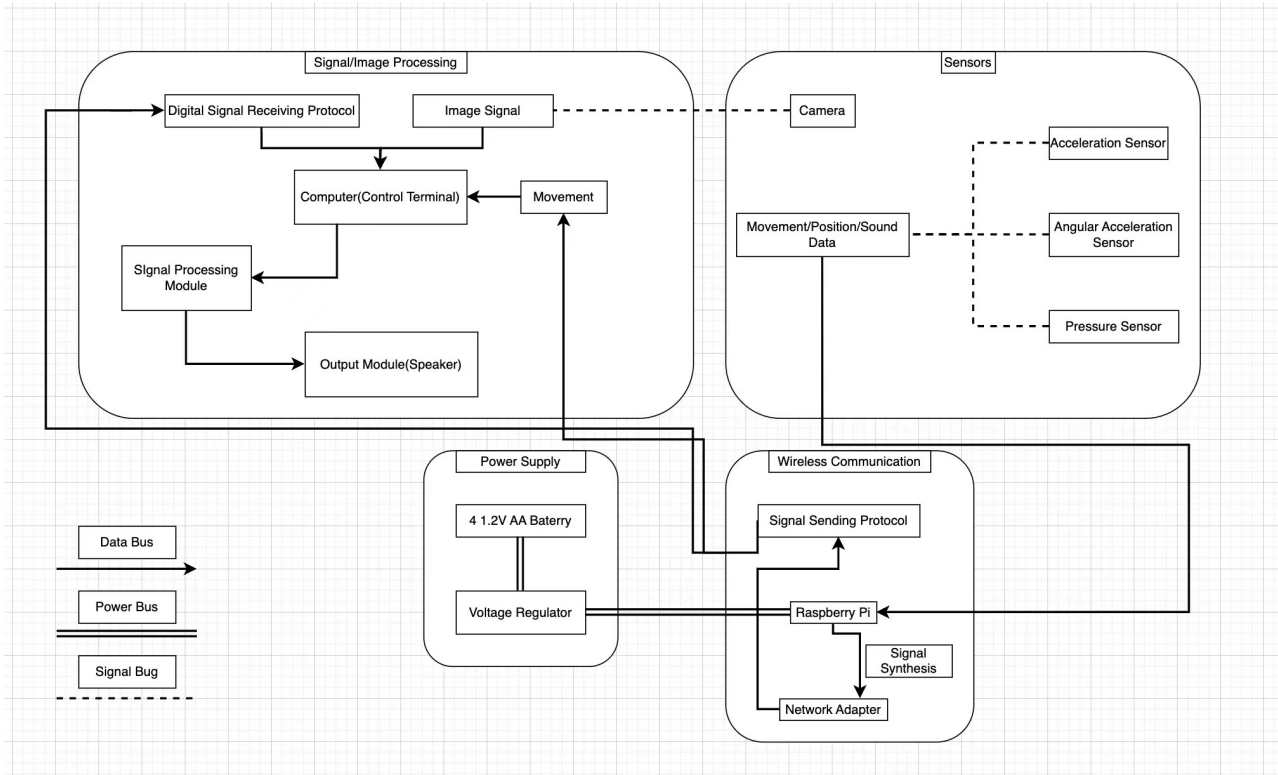
Figure 2: Block Diagram for Virtual Band Gloves[1]
