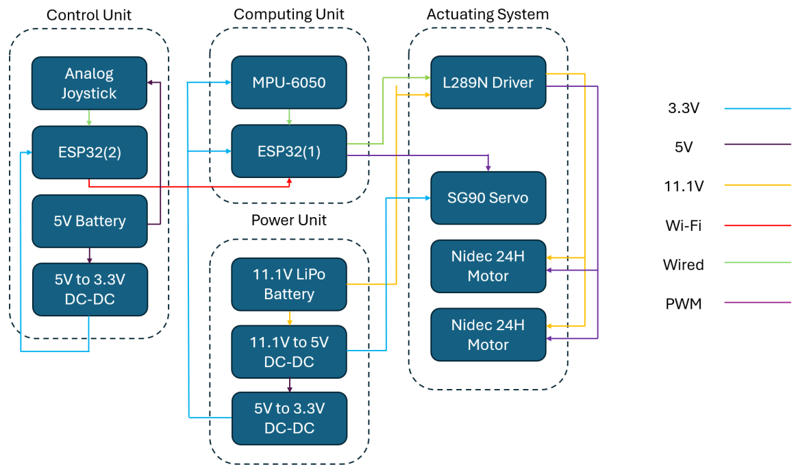
Figure 2: Block Diagram
