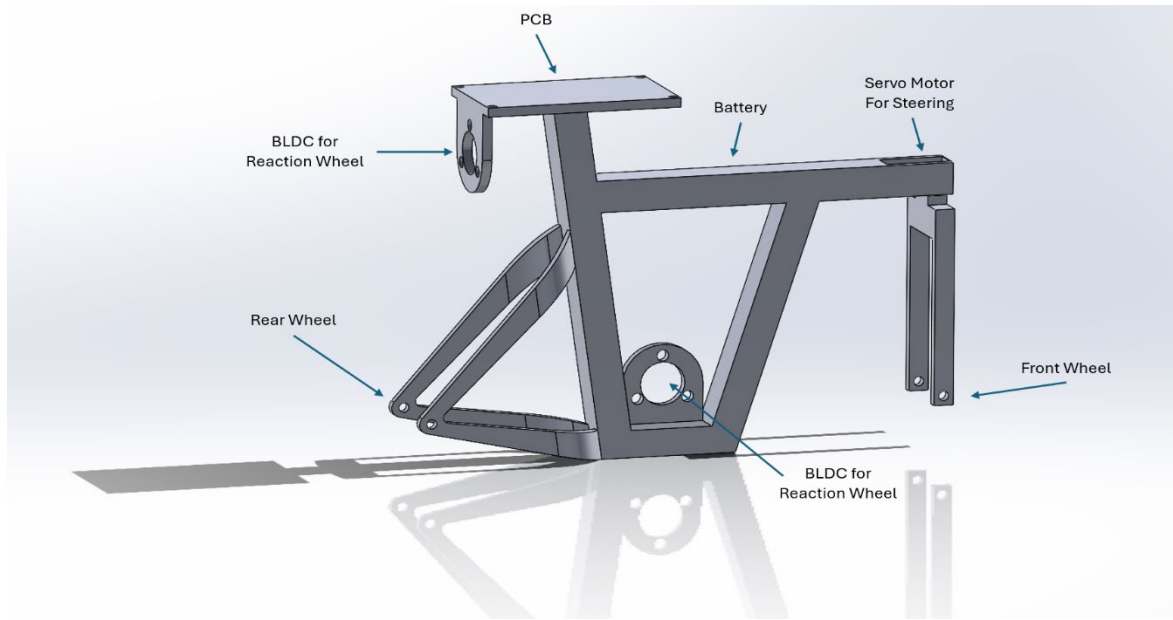
Figure 3: Physical Design
