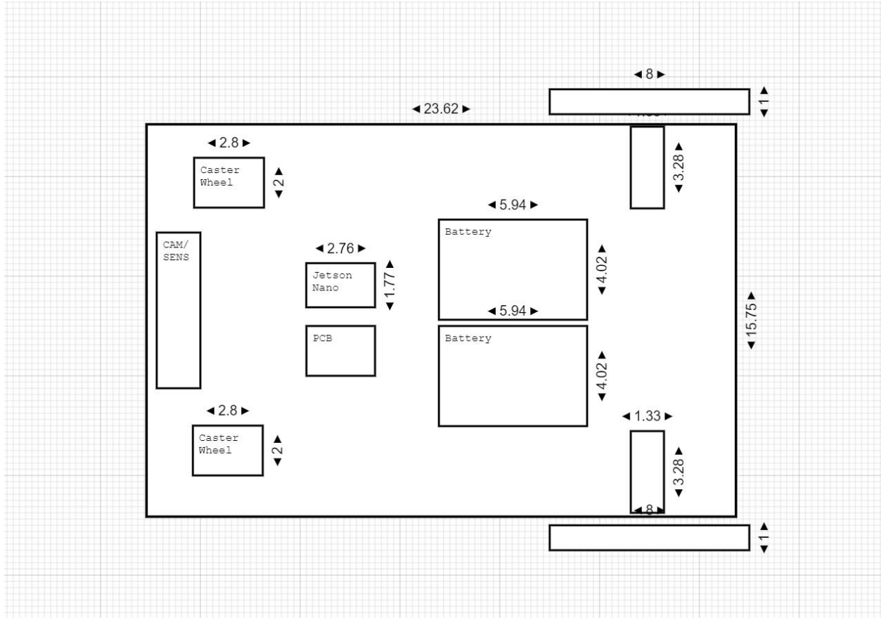
Figure 2: Mechanical Sketch (Looking from the bottom)
