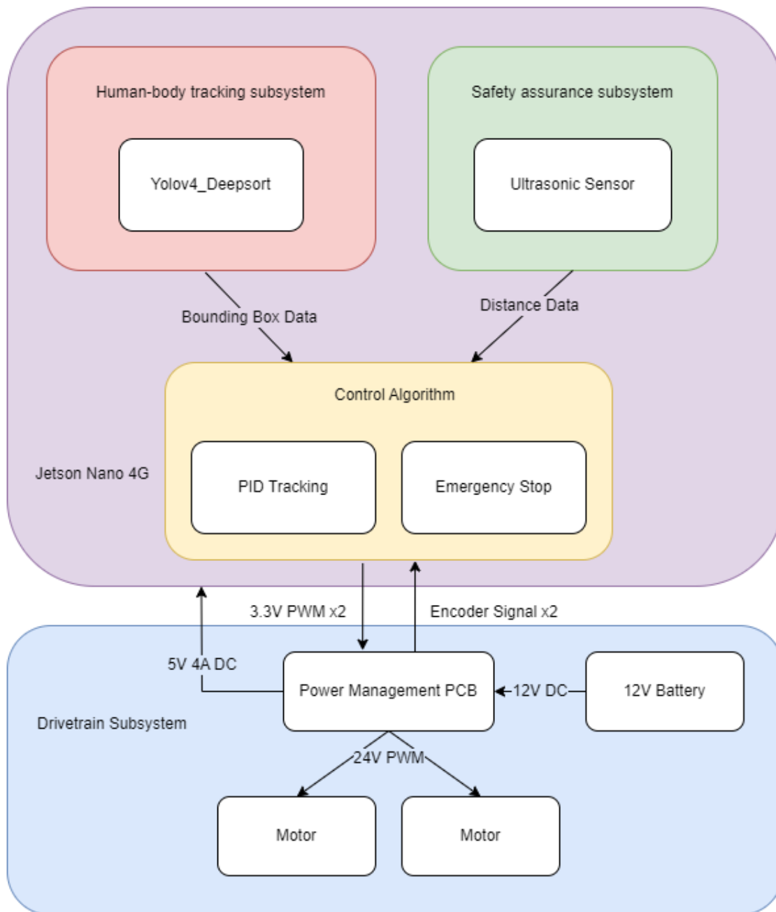
Figure 2: Block Diagram
