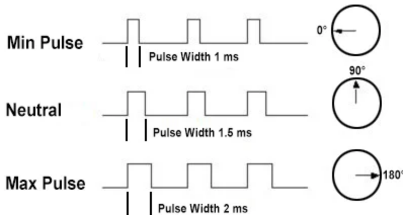
Figure 14: Servo Motor PWM Diagram
