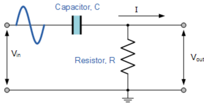
Figure 6: High pass filter with 3-dB cutoff frequency f = 1/(2\pi RC)
