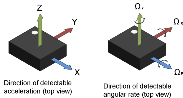
Figure 4: IMU Directions
