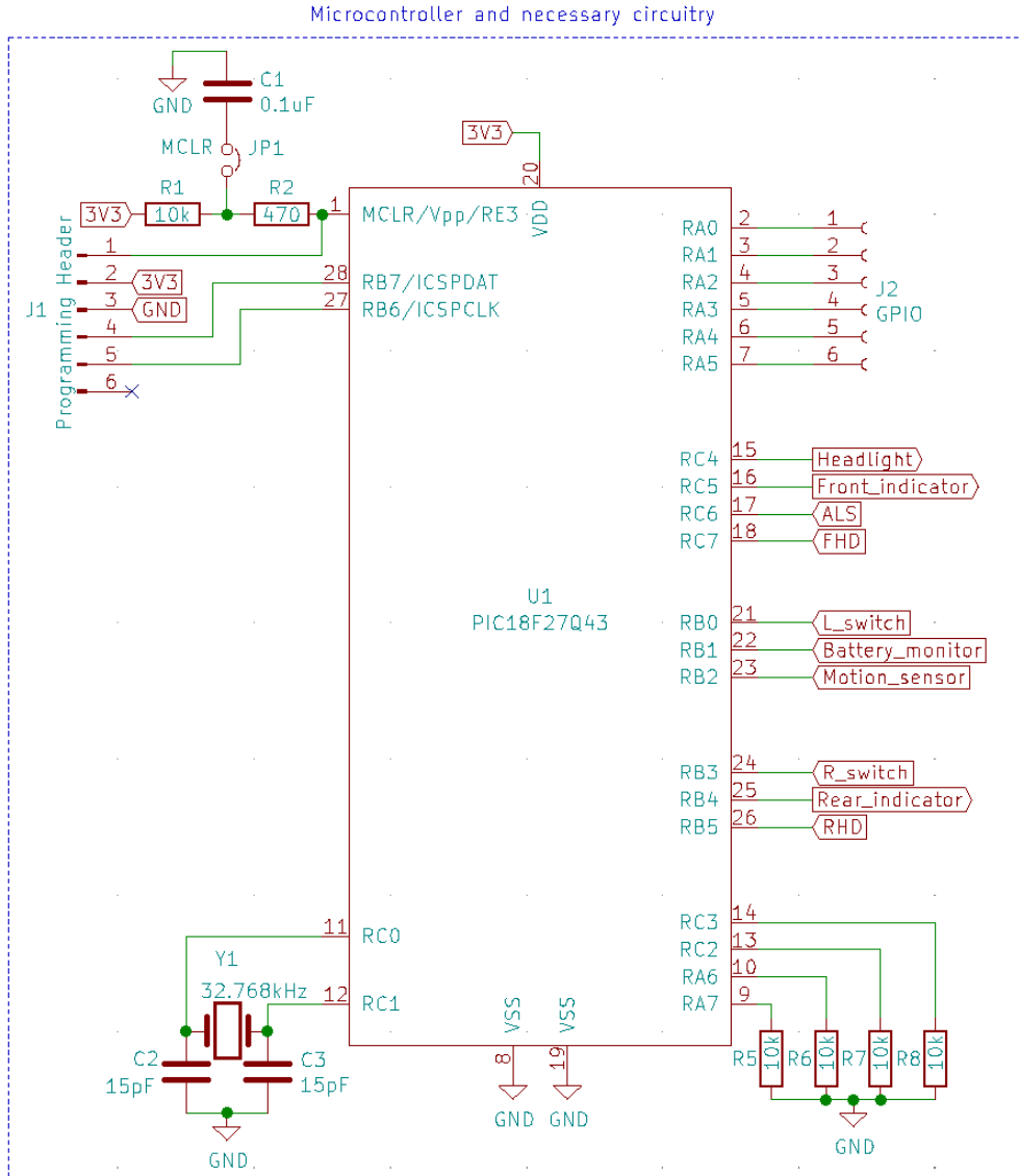
Figure 19: Microcontroller schematic
