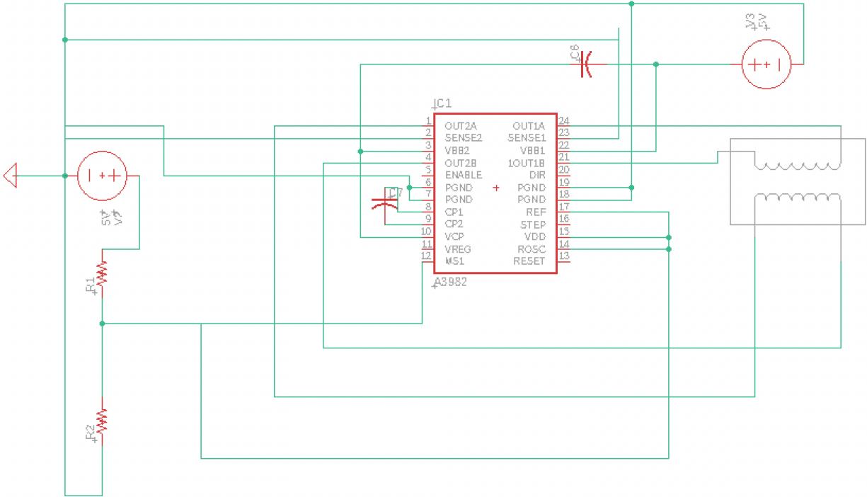
Figure 8: A3982 Driven Stepper Motor (Enable, Step, and Dir from Raspberry Pi)
