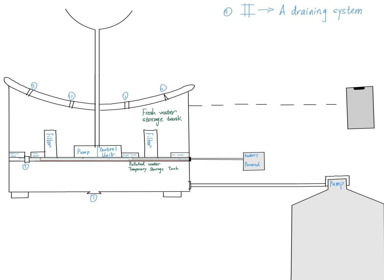
Figure 2 Smart Fountain Physical Diagram
