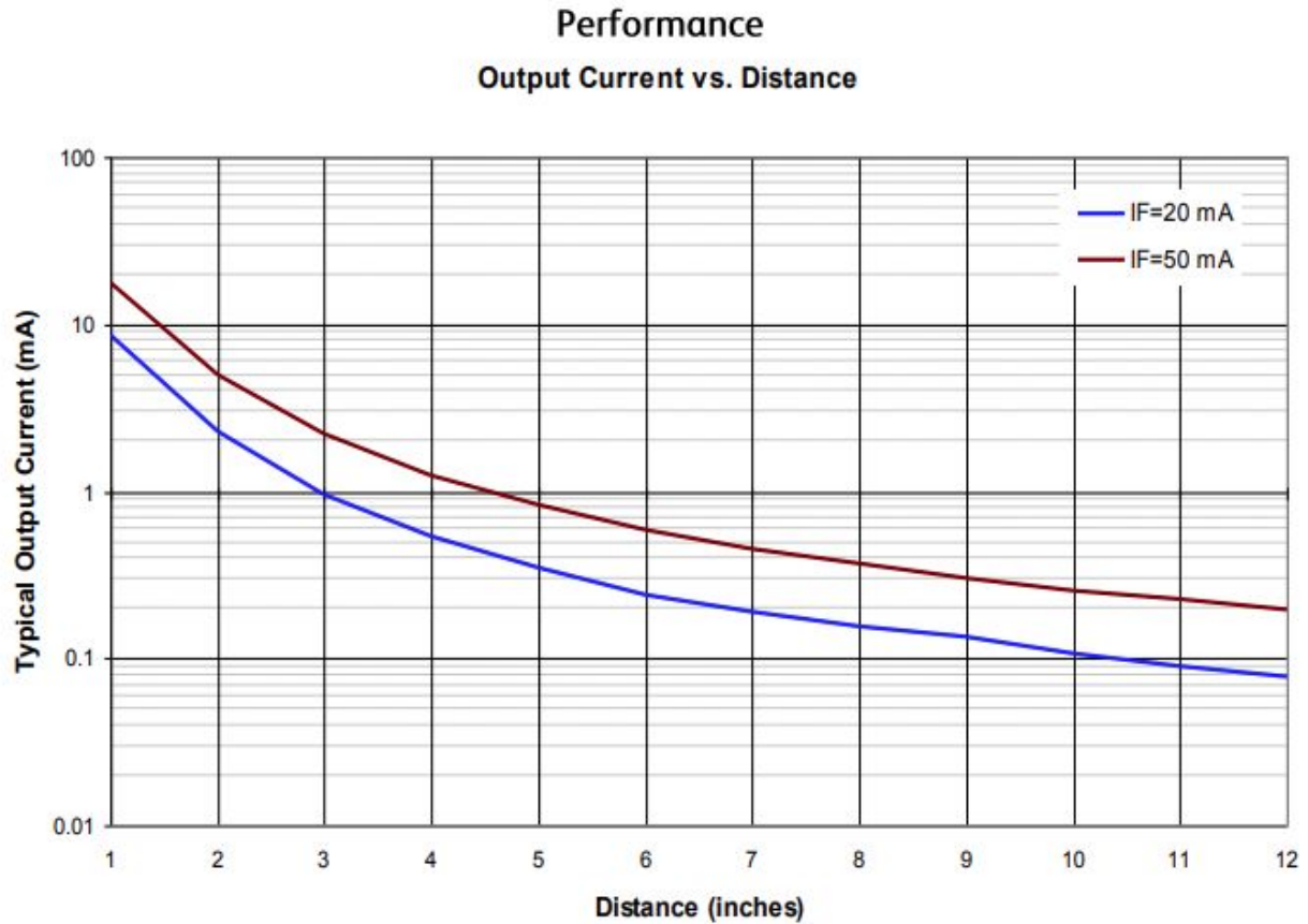
Figure 4: Current output of our Break-Beam Sensor vs. Distance from Data Sheet [5]
