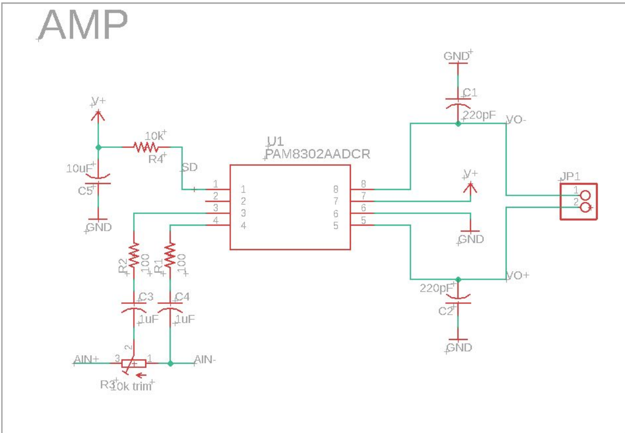
Fig. 6. Amplifier Schematic
