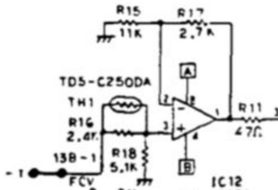
Image 9: Thermal Regulation for filter cutoff, from DW-8000 Service Manual [4]
