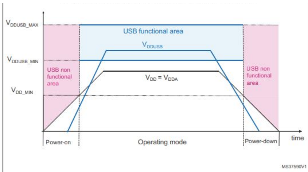
Image 10. V_{DD} , USB connected to External Power Supply [9]
