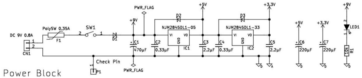
Image 4. Power Supply Diagram
