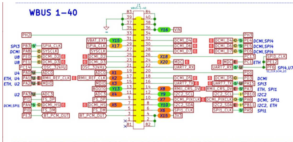
Image 5. PyBoard WBUS 1-40
