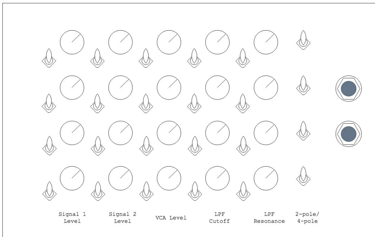
Image 2. Design Physical Layout
