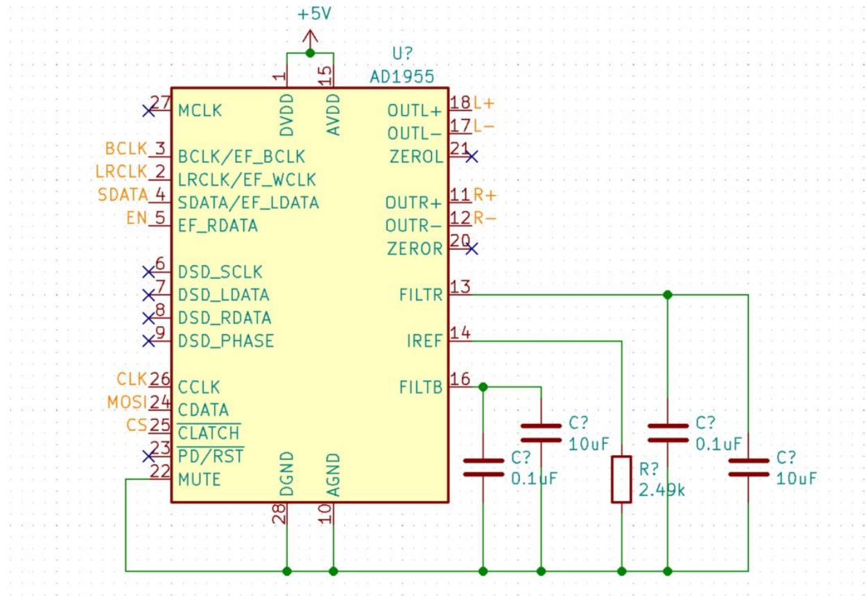
Figure 6: The digital to analog converter, or DAC, converts digital signal received from the microcontroller to an analog output that is amplified before being sent to the headphone drivers.
