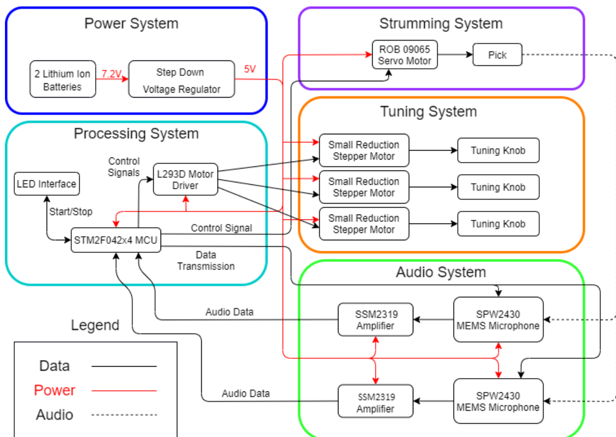
Figure 2.1 Block Diagram
