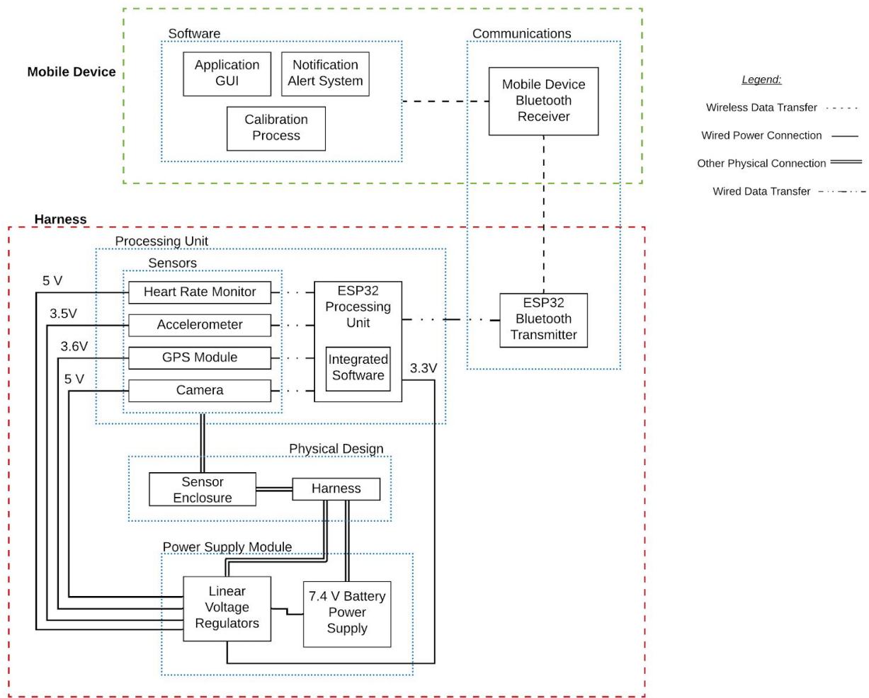
Figure 2 - Block diagram for entire project.
