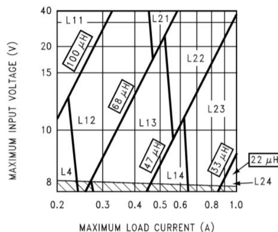
Figure 4. Inductor application curves.
