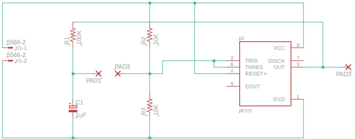
Figure 8. Turn button circuit.
