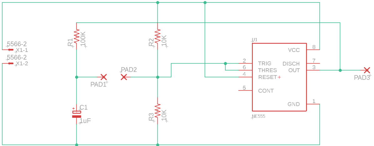
Figure 7. Turn button circuit.
