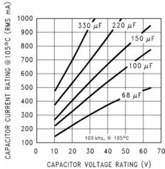
Figure 5. RMS current ratings for low ESR electrolytic capacitors (typical).
