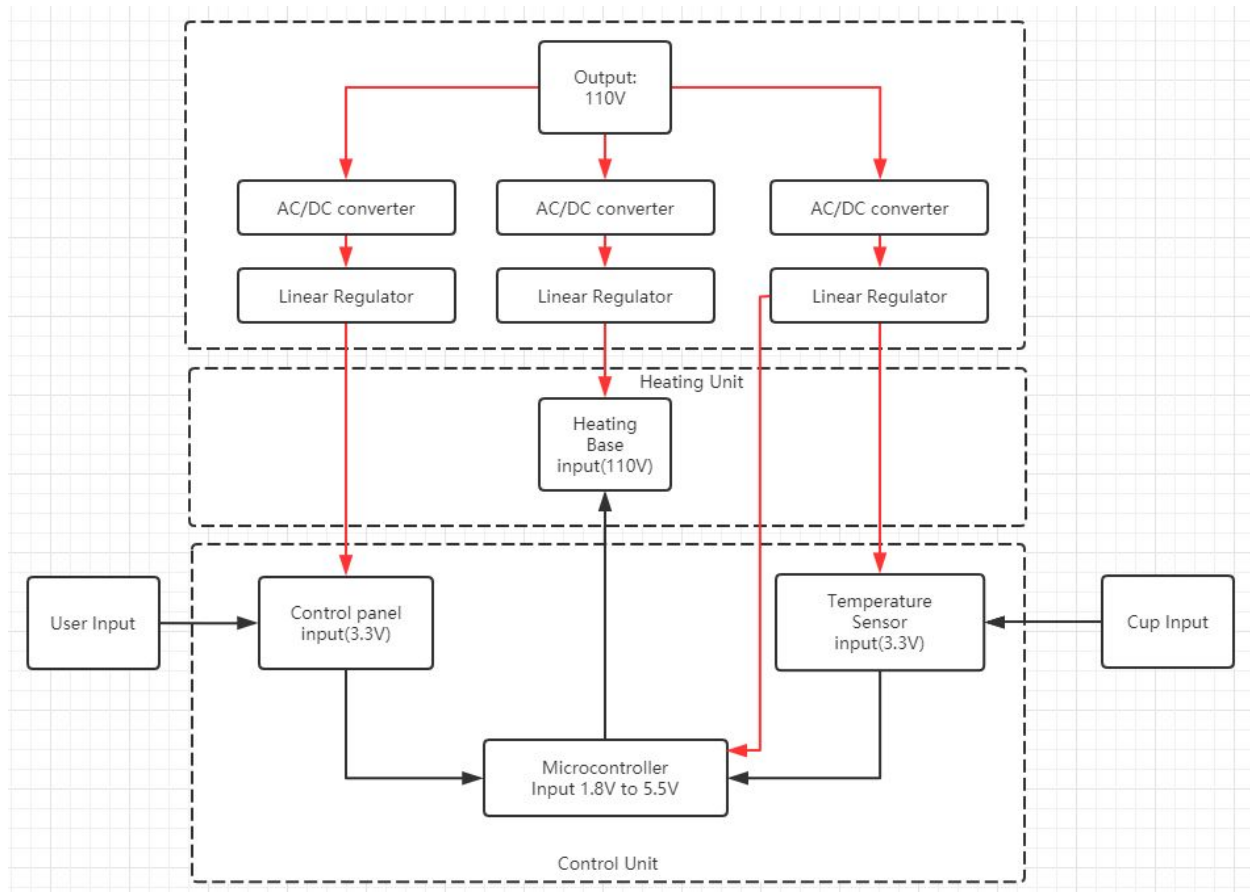
Figure 2. Block Diagram for Self-Heating Cup
