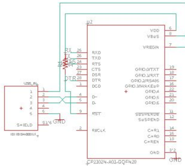
Figure 8: USB to Serial Converter Subcircuit
