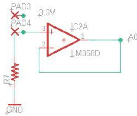
Figure 4: Flex Sensor Subcircuit Schematic
