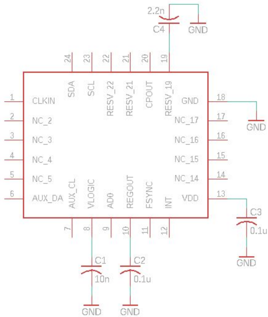
Figure 5: Accelerometer/Gyroscope Subcircuit Schematic
