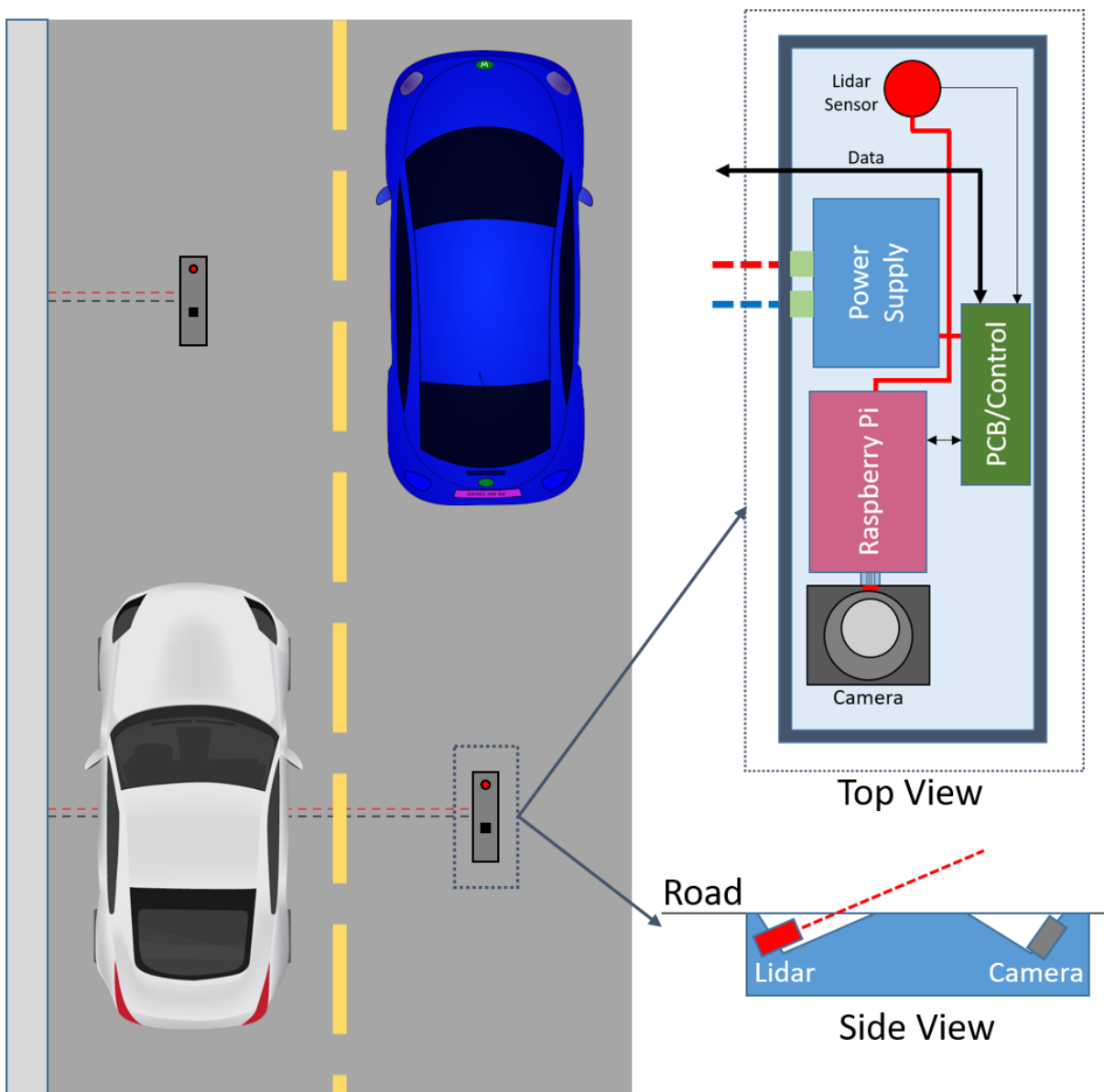
Fig. 1 - High-level graphical depiction of the design concept
