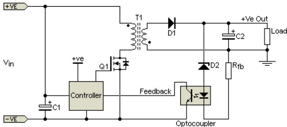
Fig. 3 - Switch-mode Flyback Power Supply, V_{in} is output of a passive bridge rectifier [7]
