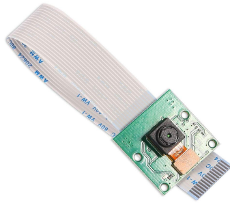
Fig. 9 - Raspberry Pi Camera Board [19]
