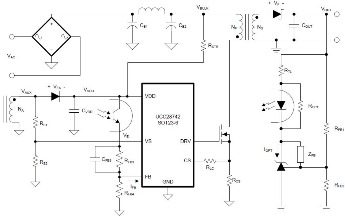
Fig. 4 - Typical application schematic from the TI UCC28742 datasheet [9]
