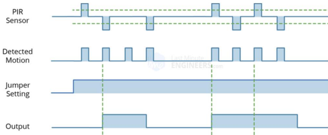
Figure 6: Timing Diagram of PIR Sensor [8]
