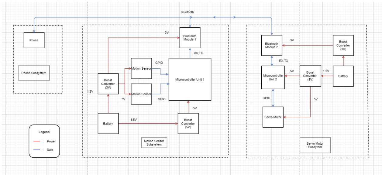
Figure 2: Block Diagram
