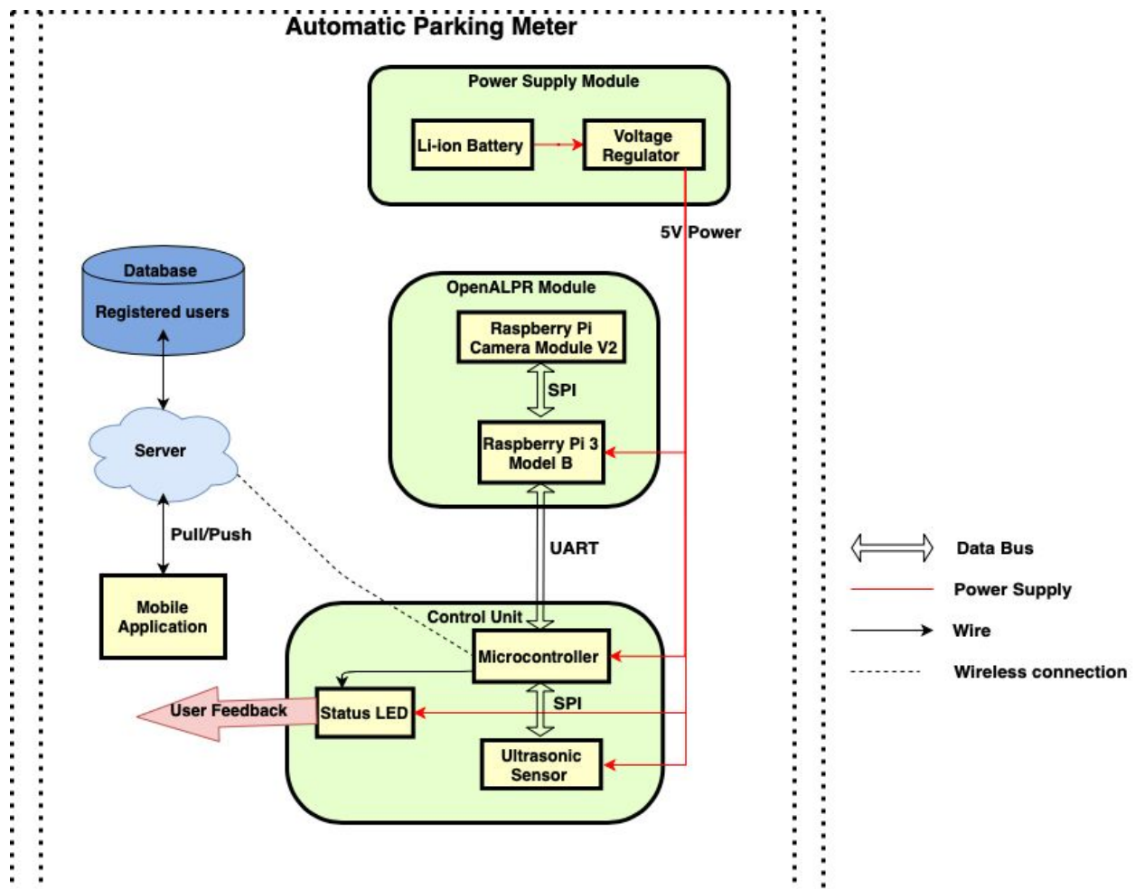
Figure 2: Automatic Parking Meter Block Diagram
