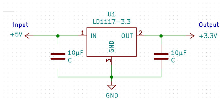
Figure 8: Circuit diagram for linear voltage regulator
