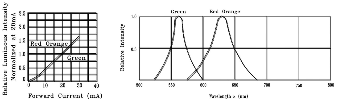
Figure 10: LED color relative to Current
