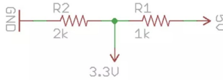
Figure 7: Circuit diagram of the voltage divider
