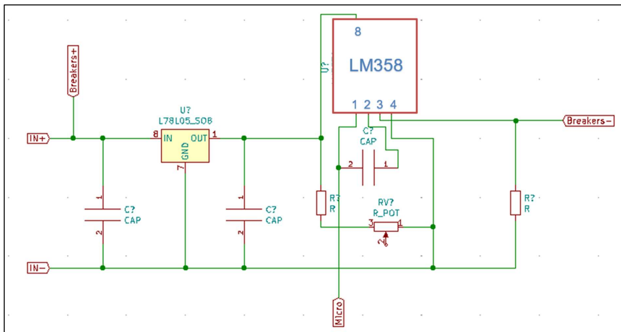
Figure 3: Current Limiter Schematic
