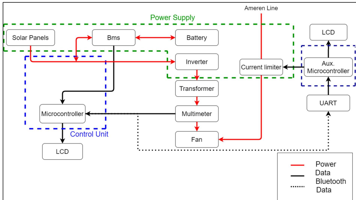
Figure 2: Block Diagram
