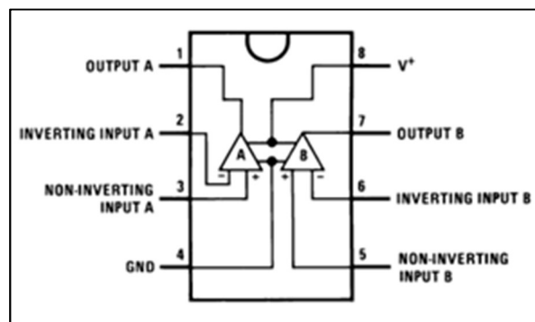
Figure 4: Pin-Planner of the LM358
