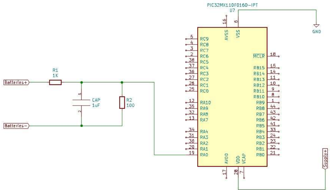
Figure 8: Voltmeter Pin Conections
