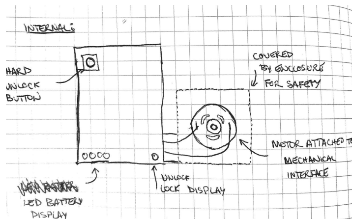
Figure 9 - Sketch of the components involved in the internal part of the locking unit. These devices will be placed on the inside of the door and electronics will be kept safely inside an enclosure. Additionally, the motor is stored here which spins the rotational component of the deadbolt.
