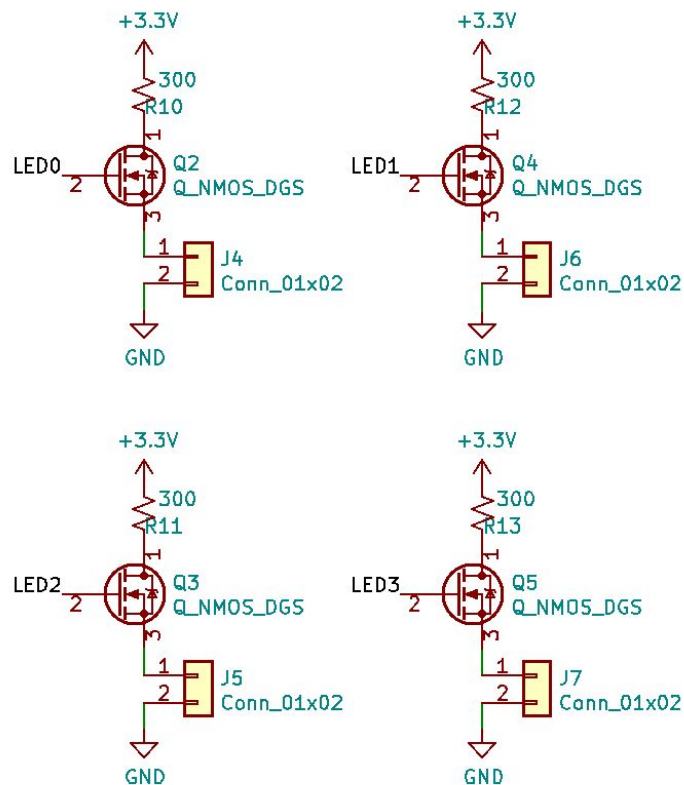
Figure 11. Floor LEDs
