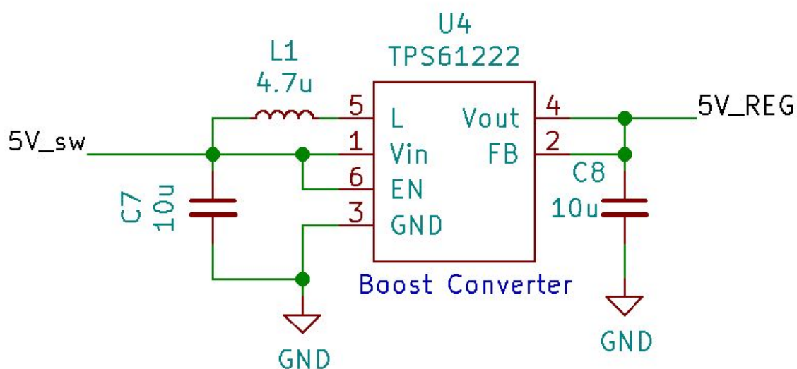
Figure 6. 5V Boost Conversion
