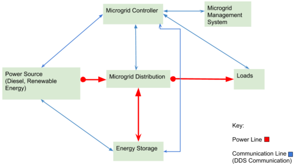
Figure 2: Block Diagram
