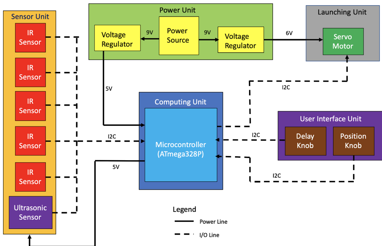
Figure 1. Block Diagram
