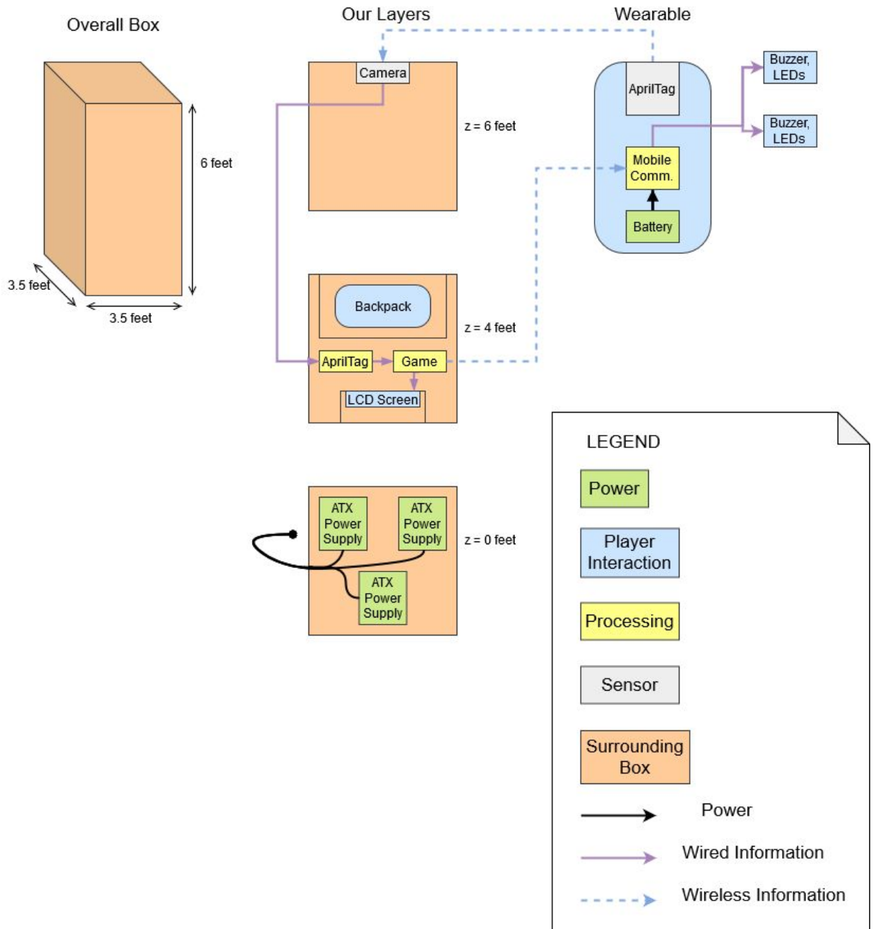
Figure 2: Physical Diagram
