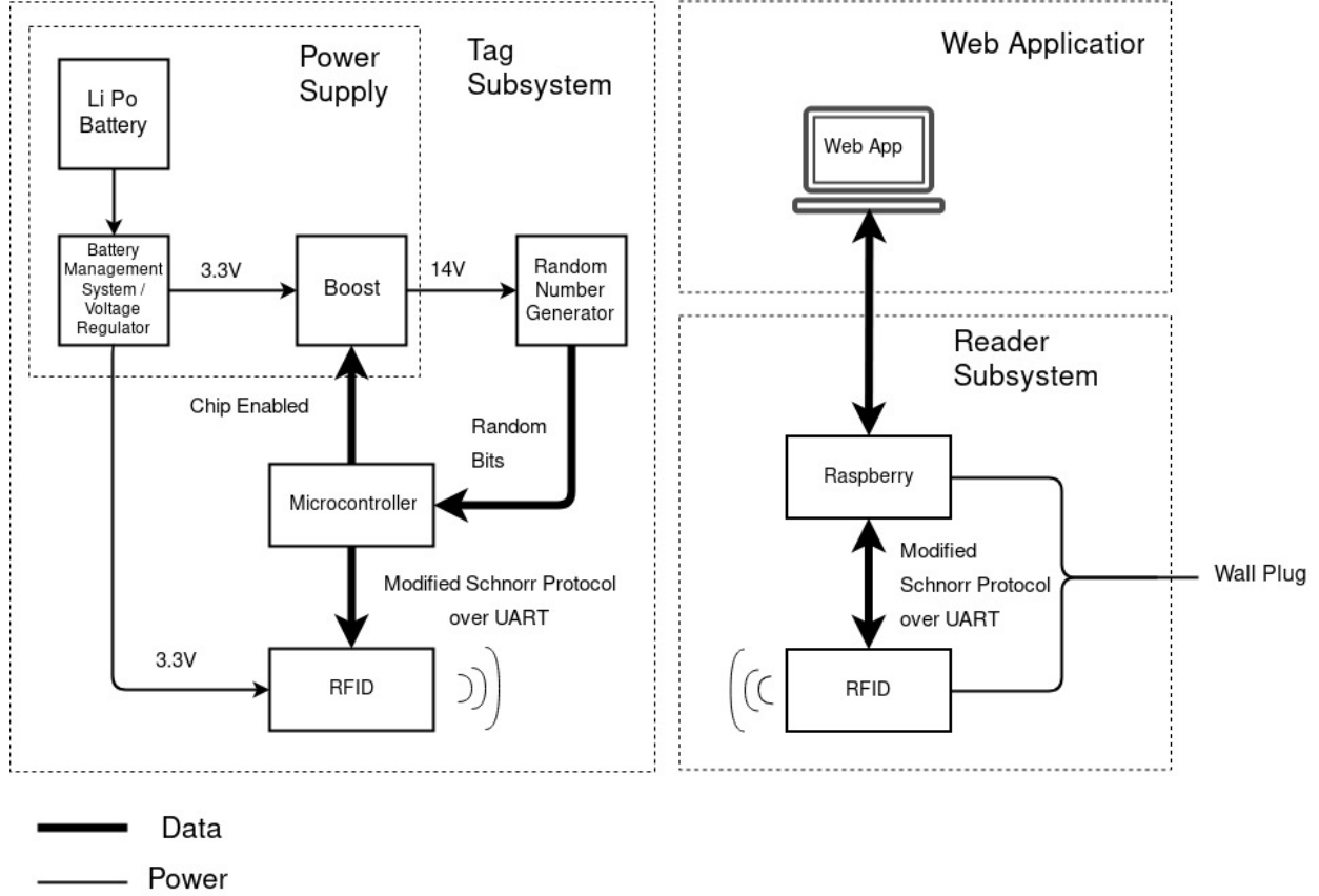
Figure 4 : Block Diagram
