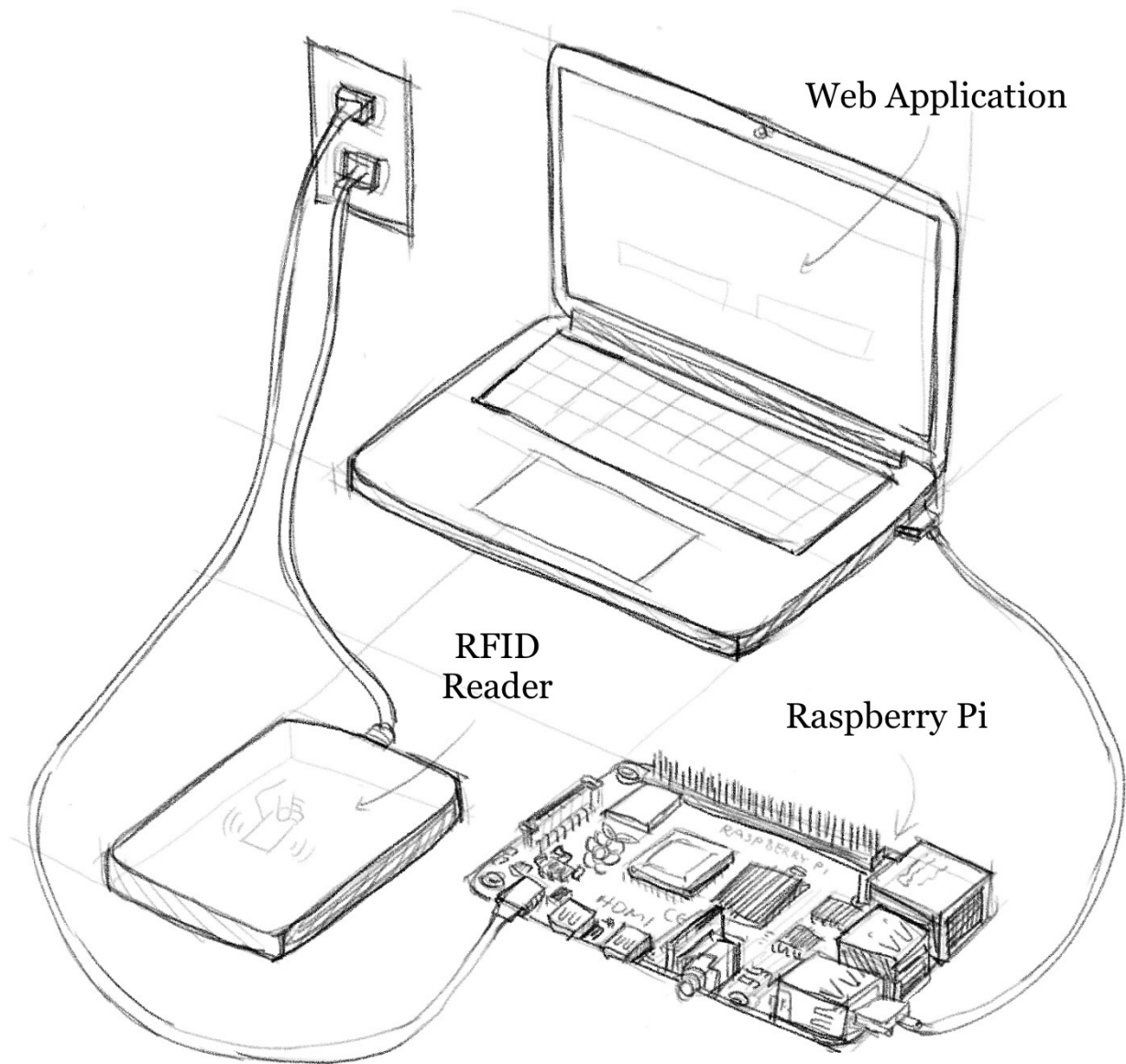
Figure 8 : Physical Reader Design
