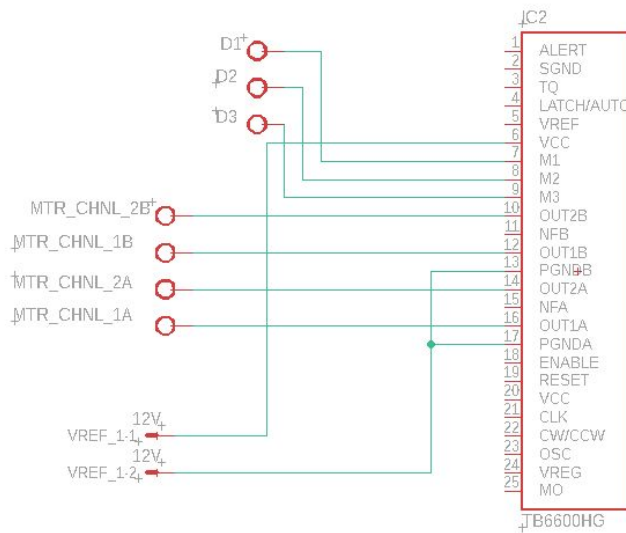
Figure 6. TB6600 Stepper Motor Driver Schematic
