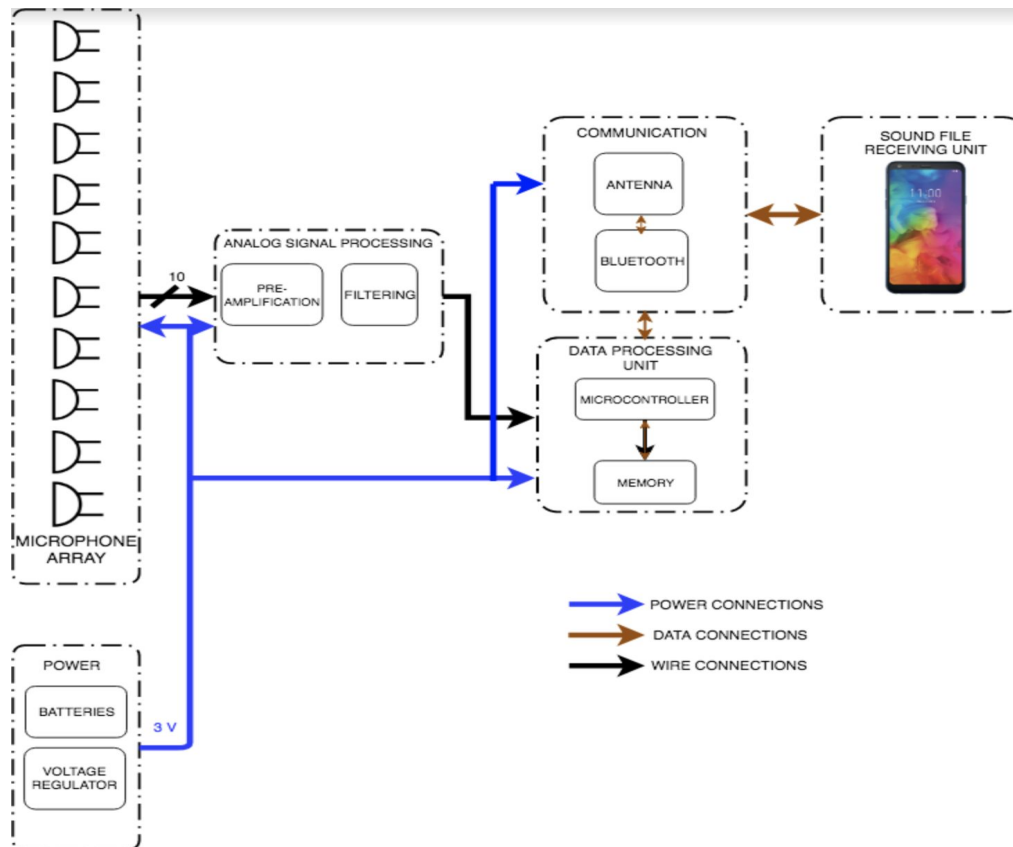
Figure 1: Block Diagram
