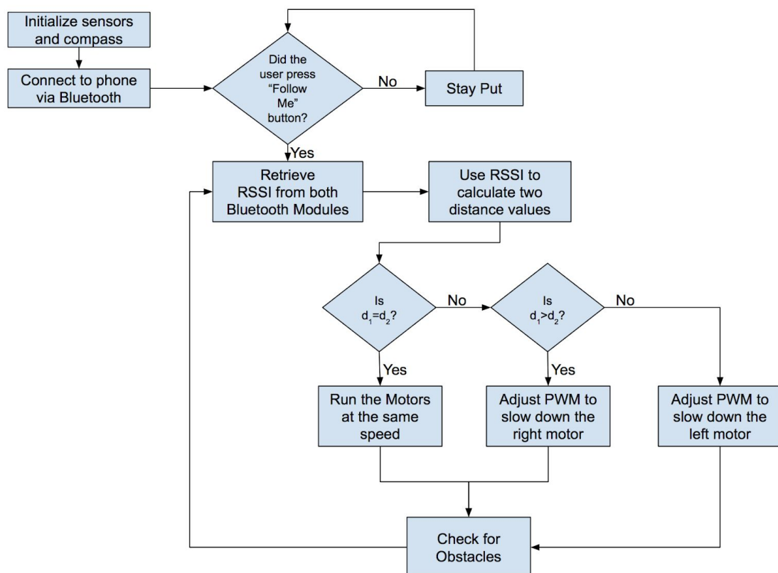
Figure 7: Software Flowchart
