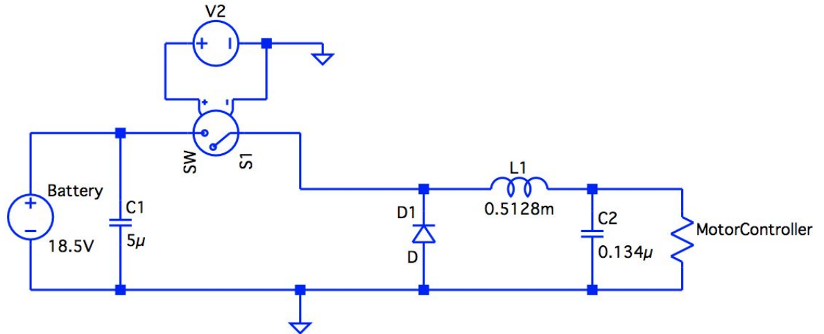
Figure 3: Voltage Regulator #1 Schematic (Buck Converter)
