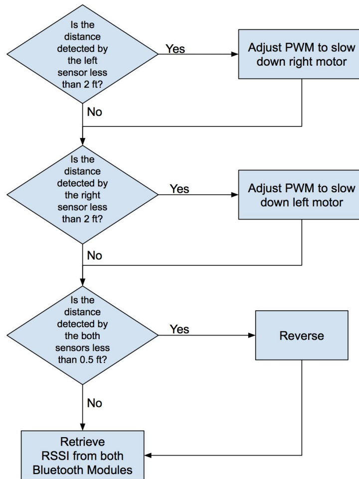
Figure 8: Obstacle Avoidance Flowchart
