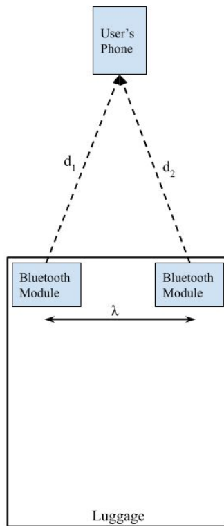
Figure 6: Bluetooth Module Placement to Calculate Distance
