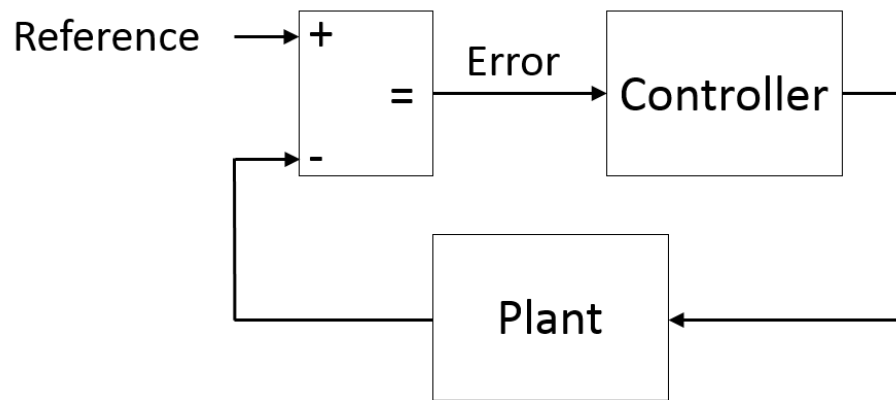
Figure 1: A generic control system involves a reference, a measure of error, a system “controller”, and a device (“plant”) to be controlled, all connected in a negative-feedback “control loop”.
