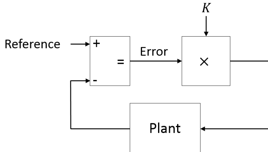
Figure 2: The simplest control system involves a reference, a measure of error, gain within the loop, and a device (“plant”) to be controlled. This is called “Proportional Control”.
