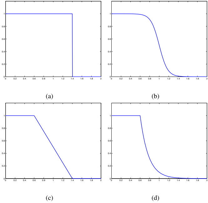
Fig. 2. Different choices for the function f . In particular, Fig. 2(a): f(y) = 1 if y \leq \rho_2 , Fig. 2(b): f(y) = \frac{1}{1+e^{-\alpha(y-\rho)}} with \alpha = \frac{2}{\rho_2-\rho_1} \log\left(\frac{1-\epsilon}{\epsilon}\right) and \rho = \frac{\rho_1+\rho_2}{2} , Fig. 2(c): f(y) = \frac{1}{\rho_1-\rho_2}y - \frac{\rho_2}{\rho_1-\rho_2} if \rho_1 \leq y < \rho_2 , and Fig. 2(d): f(y) = e^{-\alpha(y-\rho_1)} if y > \rho_1 , with \alpha = \frac{1}{\rho_2-\rho_1} \log\left(\frac{1}{\epsilon}\right) . The above plots are for \rho_1 = .6 , \rho_2 = 1.4 and \epsilon = .01 .
