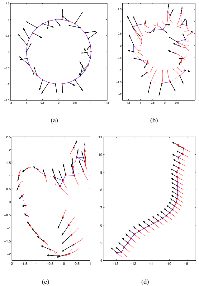
Fig. 11. Connectivity preserving flocking of n = 30 robots for a sparse initial configuration where connectivity can not be trivially maintained. It can be seen that the network remains connected while all robot velocities are asymptotically aligned. Dotted lines indicate communication links that are candidates for deletion (Fig. 10).
