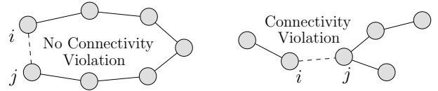
Fig. 5. Control challenges requiring knowledge of the network structure. Without such knowledge, deletion of a link (i, j) can either violate connectivity (right) or not (left).
