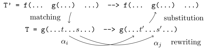
Figure 6: Behavior of matchrew
