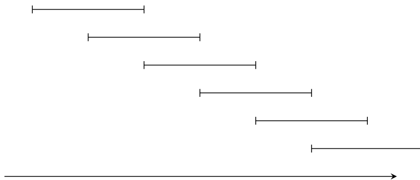
Figure: Bad instance for recursive algorithm
