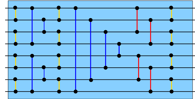
Figure: Sorter[8] .
