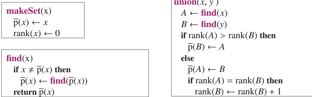
Figure 23.3: The pseudo-code for the Union-Find data-structure that uses both path-compression and union by rank. For element x , we denote the parent pointer of x by \bar{p}(x) .
