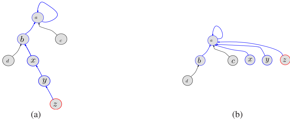
Figure 23.2: (a) The tree before performing find (z), and (b) The reversed tree after performing find (z) that uses path compression.
