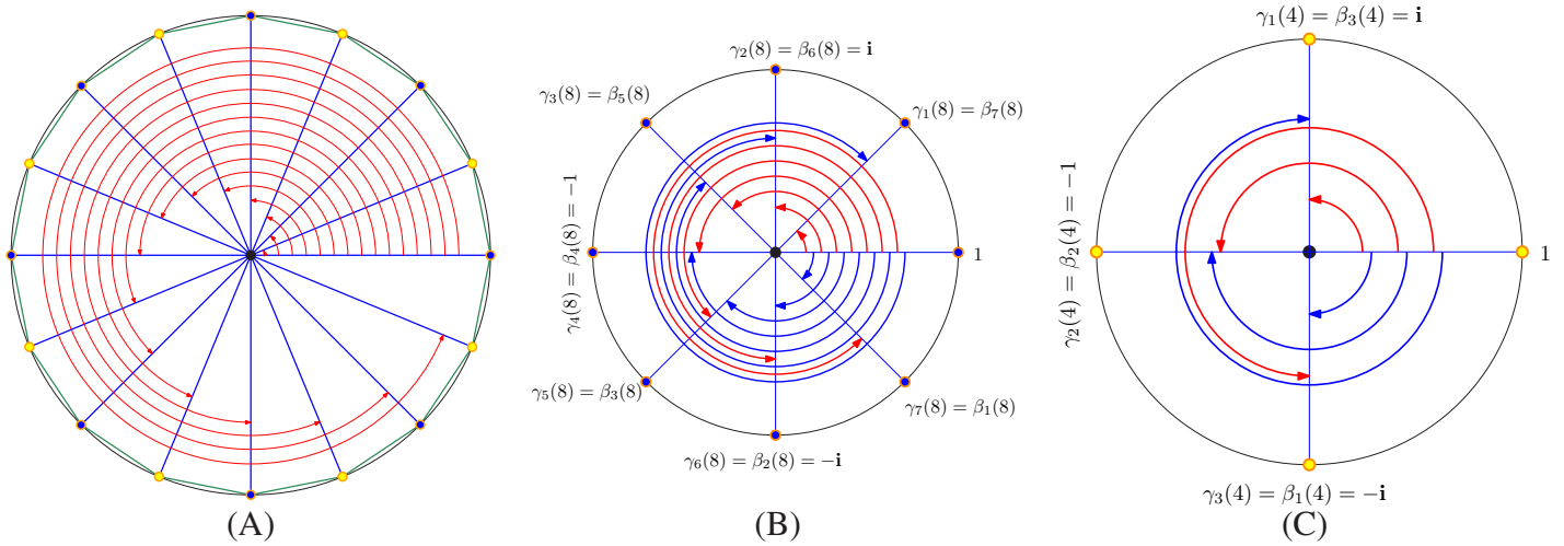
Figure 21.2: (A) The 16 roots of unity. (B) The 8 roots of unity. (C) The 4 roots of unity.
