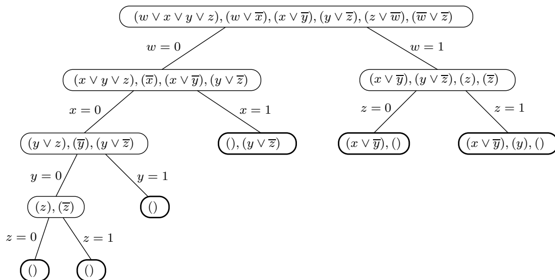
Figure: Backtrack search. Formula is not satisfiable.
