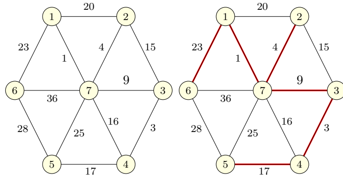
Figure 12.1: Graph with unique edge costs. Safe edges are red, rest are unsafe.
