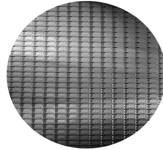
Figure 1.15 This 300 mm wafer contains 280 full Sandy Bridge dies, each 20.7 by 10.5 mm in a 32 nm process. (Sandy Bridge is Intel's successor to Nehalem used in the Core i7.) At 216 mm 2 , the formula for dies per wafer estimates 282. (Courtesy Intel.)
